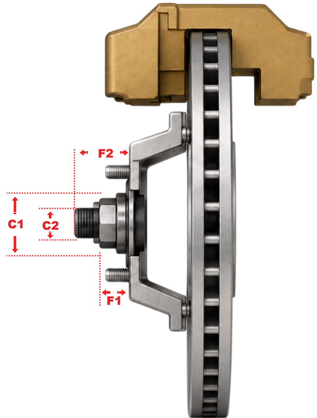
Hub & Axle 2D Side View
